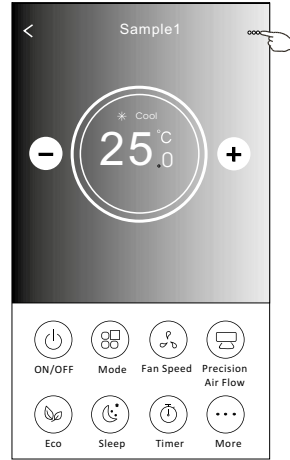
Control form2
